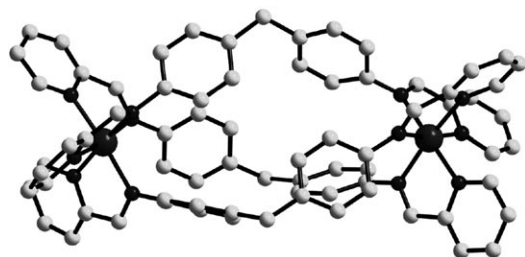
Figure 1. Structure of [\text{Ru}_2\text{L}_3]^{4+} cation. Ru large black spheres, N small black spheres, C small gray spheres. Hydrogen atoms, anions, and cocrystallized solvent molecules are omitted for clarity.
